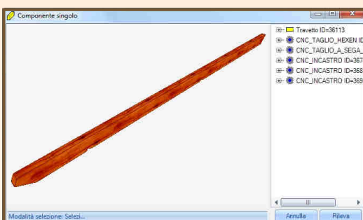
3D Machining Inspector
