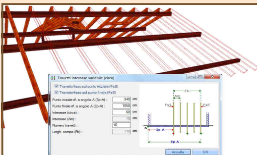
Free rafters arrangement
