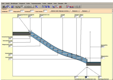
Stringer Side View Quarter Turn Stair-
